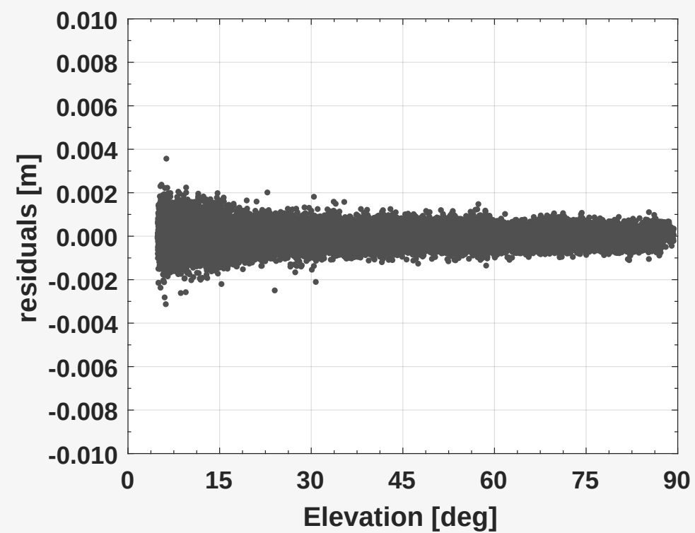
(a) GL1C-GL2X
