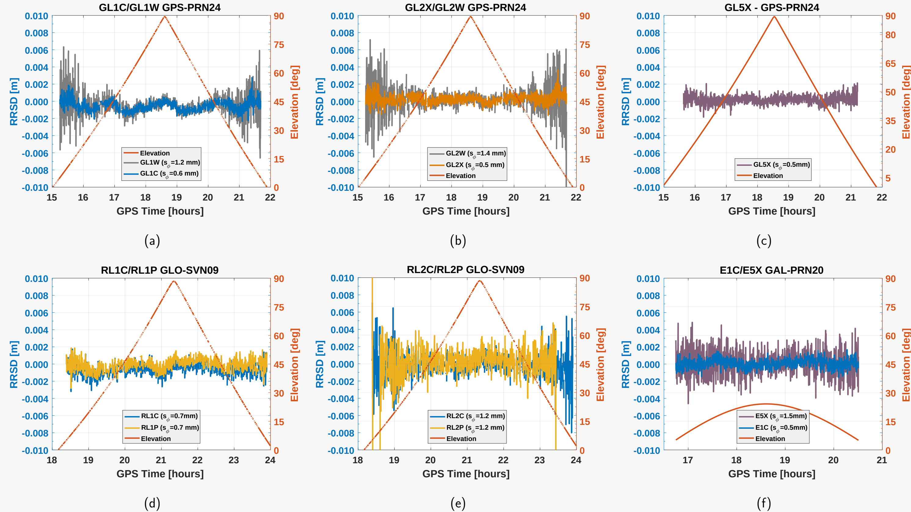
Figure 2: Individual RRSD for various GNSS, signals and modulations shown exemplary for individual satellites, (a-c) GPS, (d-e) GLONASS and (f) Galileo. Individual standard deviations ( s_0 ) of RRSD indicate precise observations and a stable repeatability. Individual offsets removed for comparison reasons. Variations of the single differences origin from both, environmental conditions inside the laboratory and corresponding (possible) delays in the cables from the splitter. RRSD refer to the baseline JAV3-JAV1.
