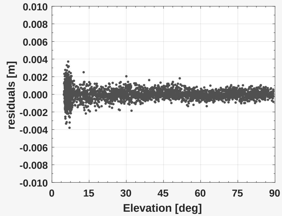
(b) GL1C-GL5X
