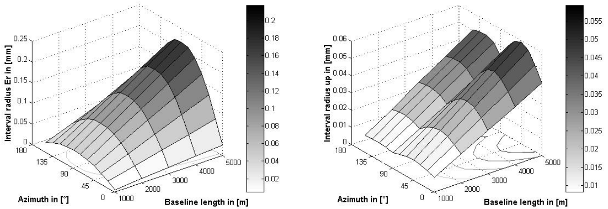
Figure 1: Interval radii for the east component (left) and height component (right) in mm
