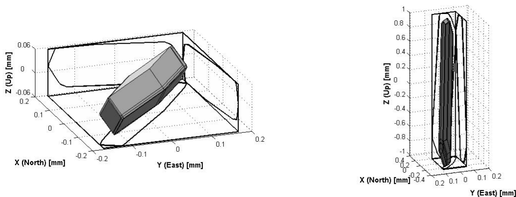
Figure 3: Zonotopes describing the factual range of coordinate imprecision for the endpoint of a 5 km baseline oriented in azimuth 45°.
