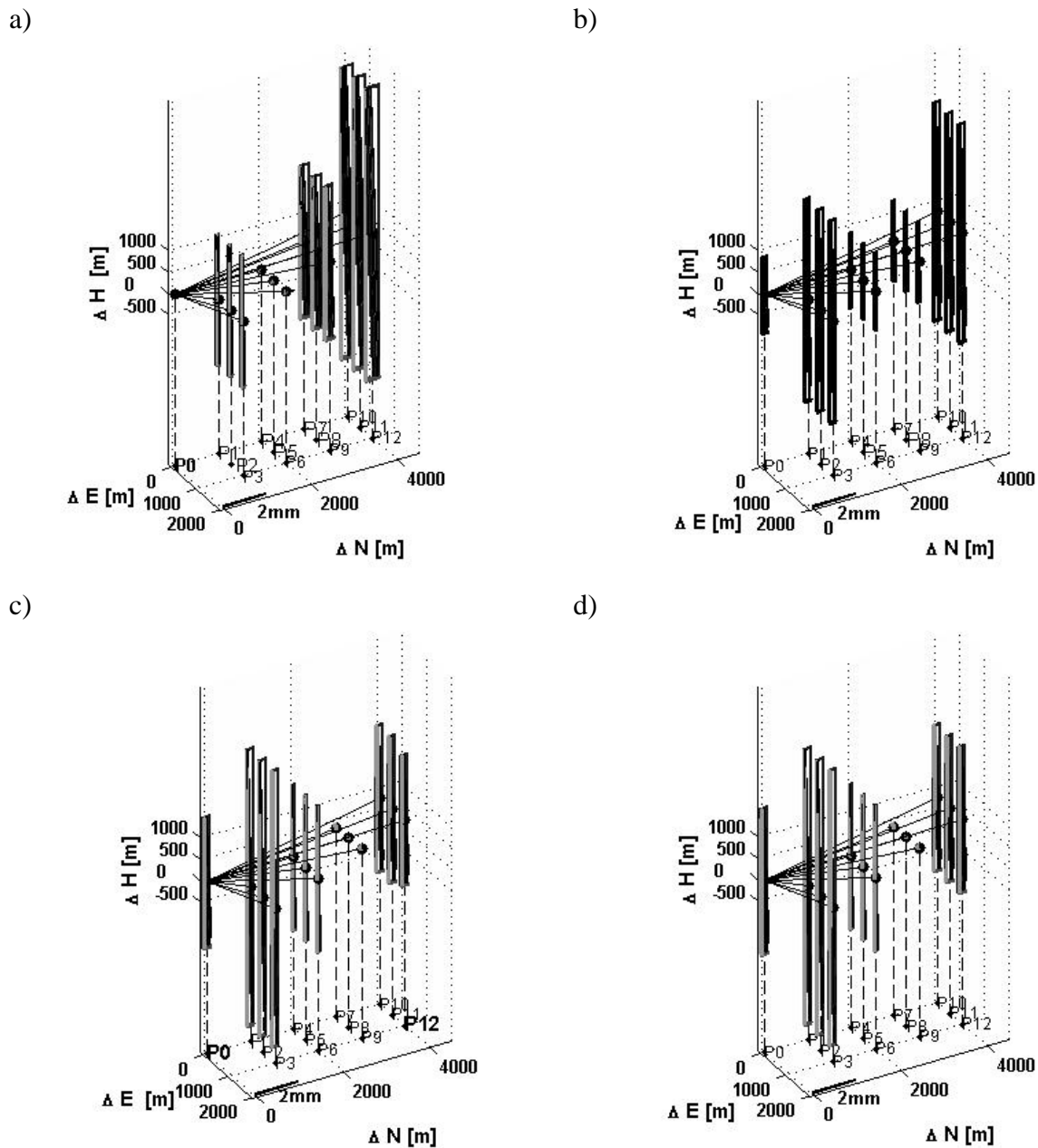
Figure 5: Variation of the size and the shape of the zonotopes applying different strategies to stabilise the normal equation
