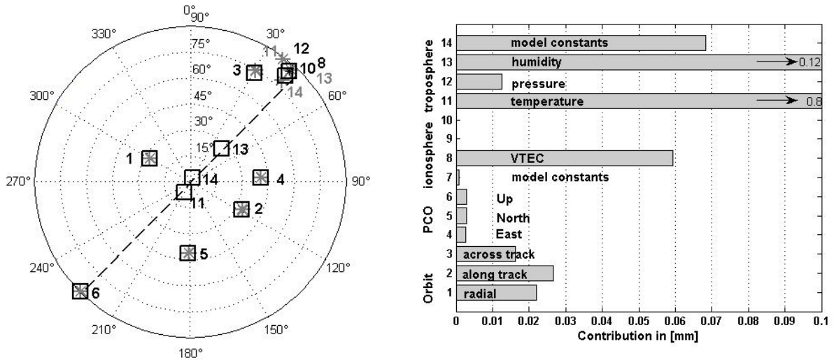
Figure 4: Contribution of basic influence parameters to the coordinate imprecision Left: Azimuth-elevation diagram of the directions of contribution(dashed line: baseline, light grey asterisks: zero height differences, black squares: height difference of 100 m) Right: Magnitude of the contributions in mm
